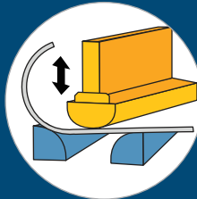
③ JCO FORMING PRESS
