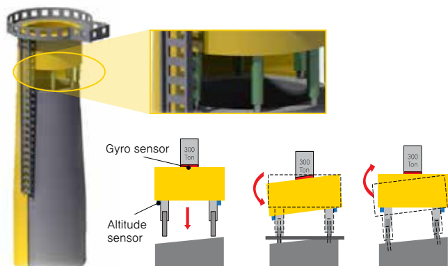
Hydraulic cylinder synchronization control mechanism
